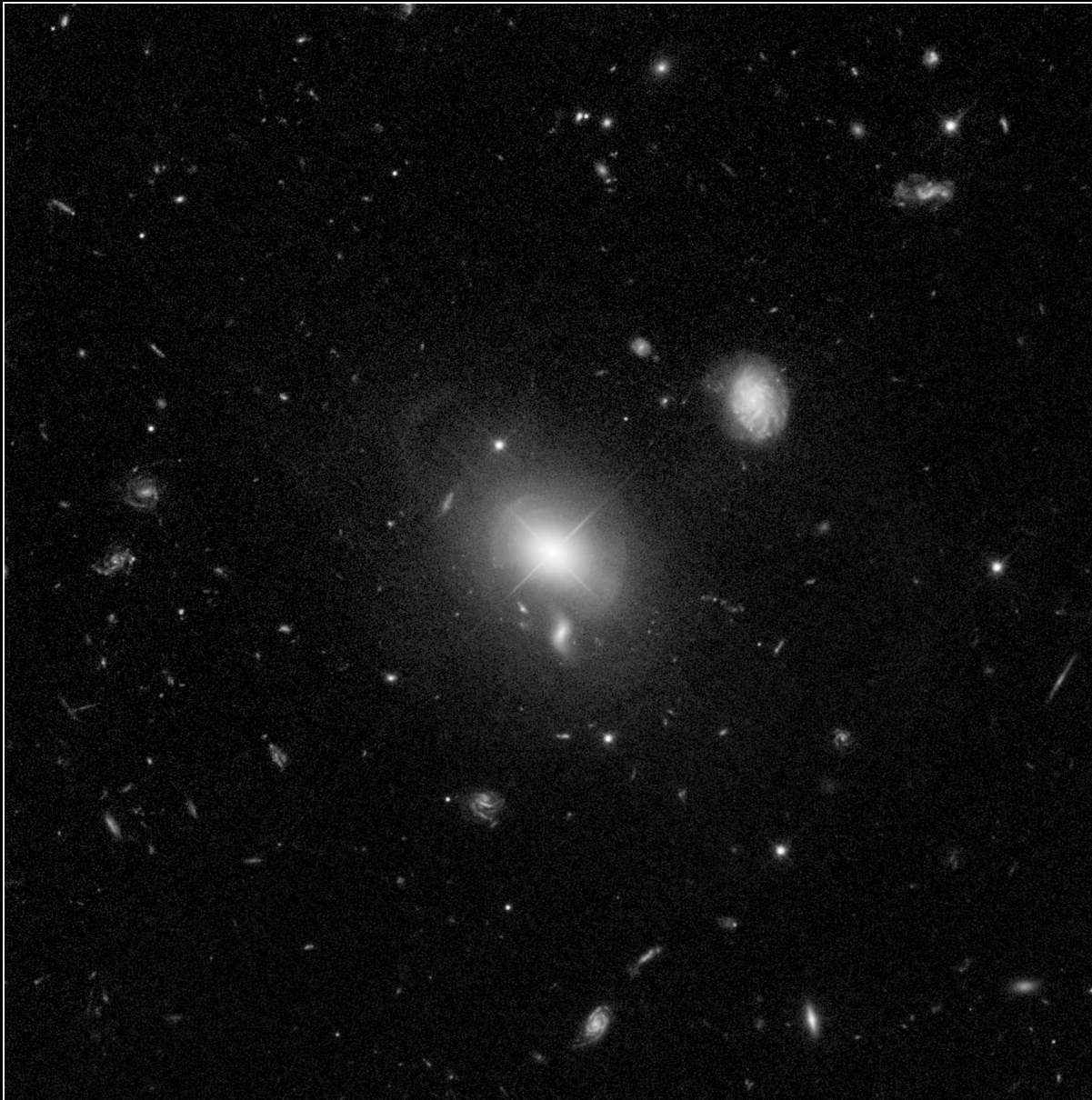
QSO MC2 1635+119 Hubble Space Telescope • ACS/WFC
