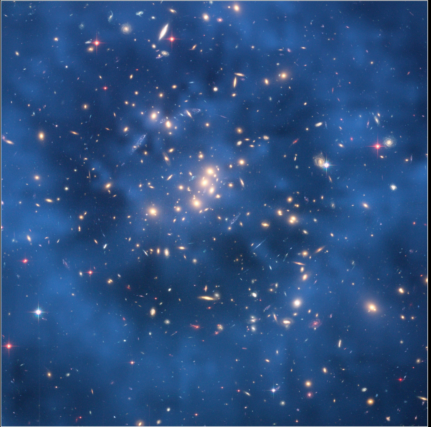
Dark Matter Ring in Galaxy Cluster CI 0024+17 (ZwCl 0024+1652) Hubble Space Telescope • ACS/WFC
