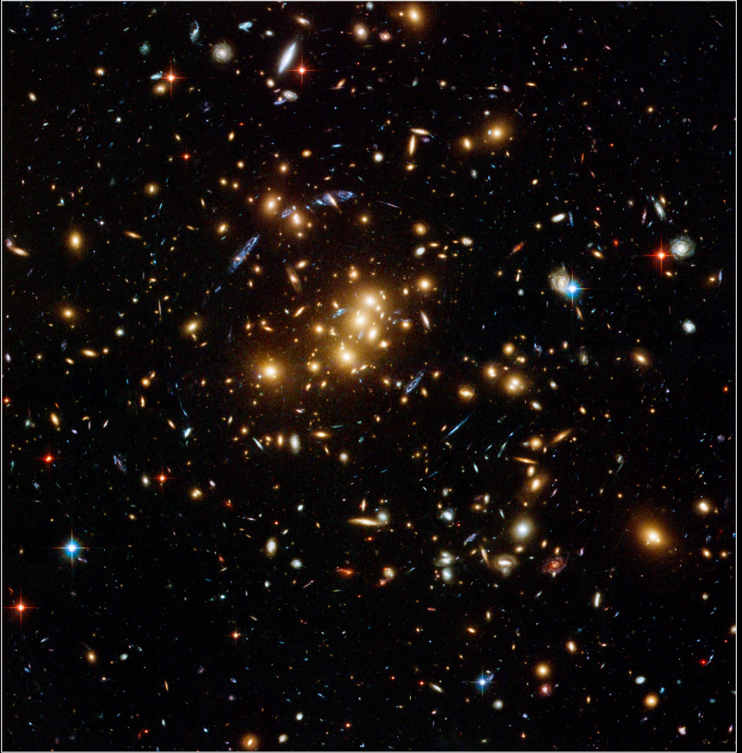
Galaxy Cluster CI 0024+17 (ZwCI 0024+1652) Hubble Space Telescope • ACS/WFC
