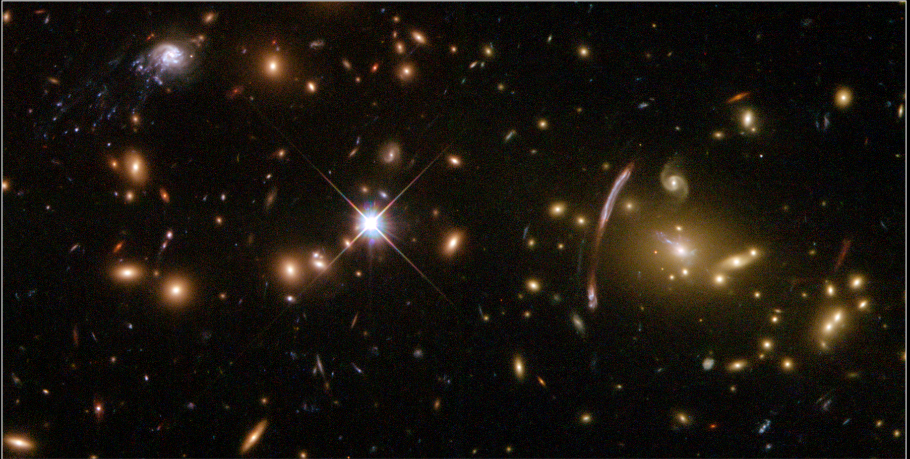
Galaxy Cluster Abell 2667 Hubble Space Telescope • WFPC2
