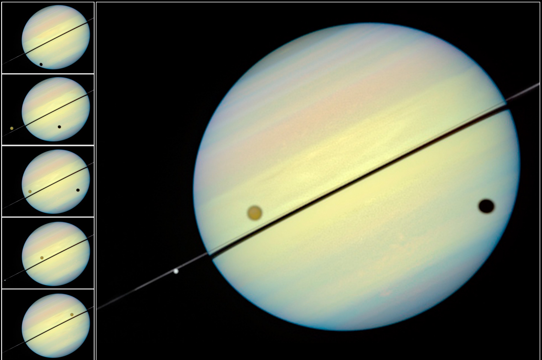
Saturn • August 6, 1995 Hubble Space Telescope • WFPC2
