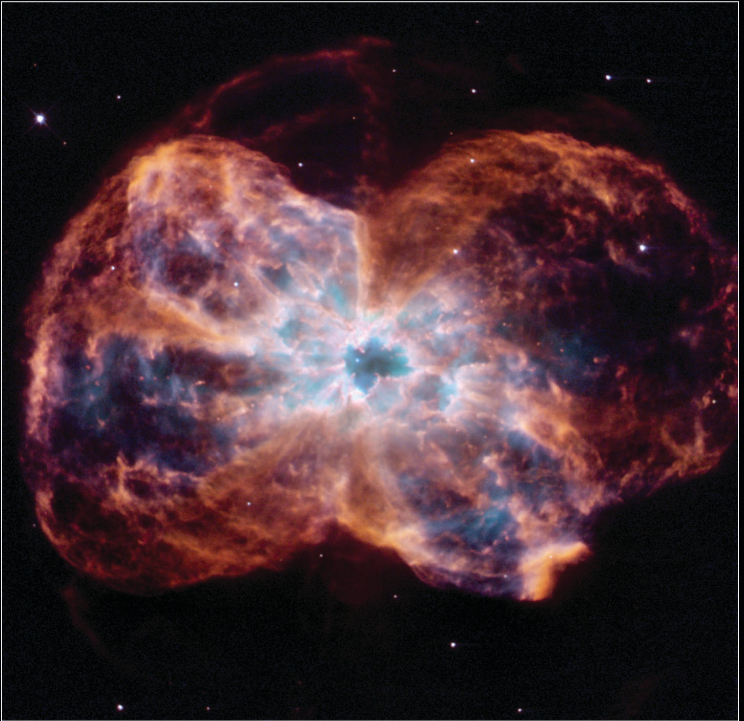
Planetary Nebula NGC 2440 Hubble Space Telescope • WFPC2
