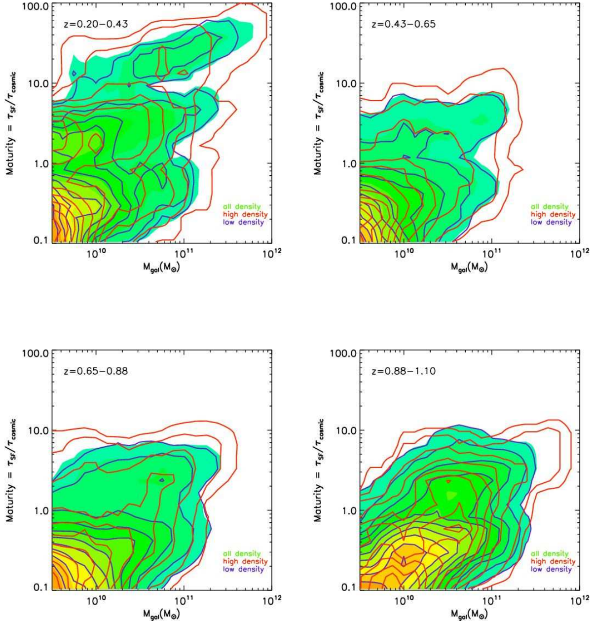
Fig. 21.— The Maturity ( = \tau_{SF}/\tau_{cosmic} ) is shown as a function of galactic mass for high and low density environments. The cut between high and low density was taken at relative density \rho = 45 , i.e. between the middle two bins of the 4 density bins used earlier. The overall distribution of galaxies is shown with the shaded area while the high and low density environments are shown separately by the red and blue contours, respectively. M < 1 correspond to active, star forming galaxies and M > 1 corresponds to galaxies which formed most of their stars at earlier epochs but see text for a more detailed discussion for interpretation of the Maturity.
