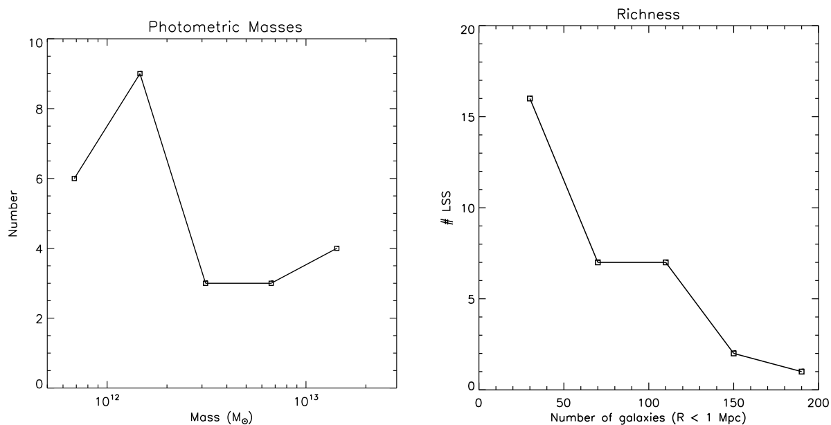
Fig. 8.— a) Left : The distribution of total stellar masses for the structures are shown for masses 5 \times 10^{11} to 10^{14} M_{\odot} . b) Right : The distribution of Richness measures for the the structures is shown, calculated as the surface density of galaxies brighter than 2 mag below the 3rd brightest galaxy (see text). Specifically, Richness is defined as the number of galaxies within the central R \leq 1 Mpc brighter than 2 magnitudes fainter than the 3rd brightest galaxy within the cluster (i.e. M_V < M_V(3rd) + 2 ). Radius is measured from the location of peak surface density as in Figure 7.
