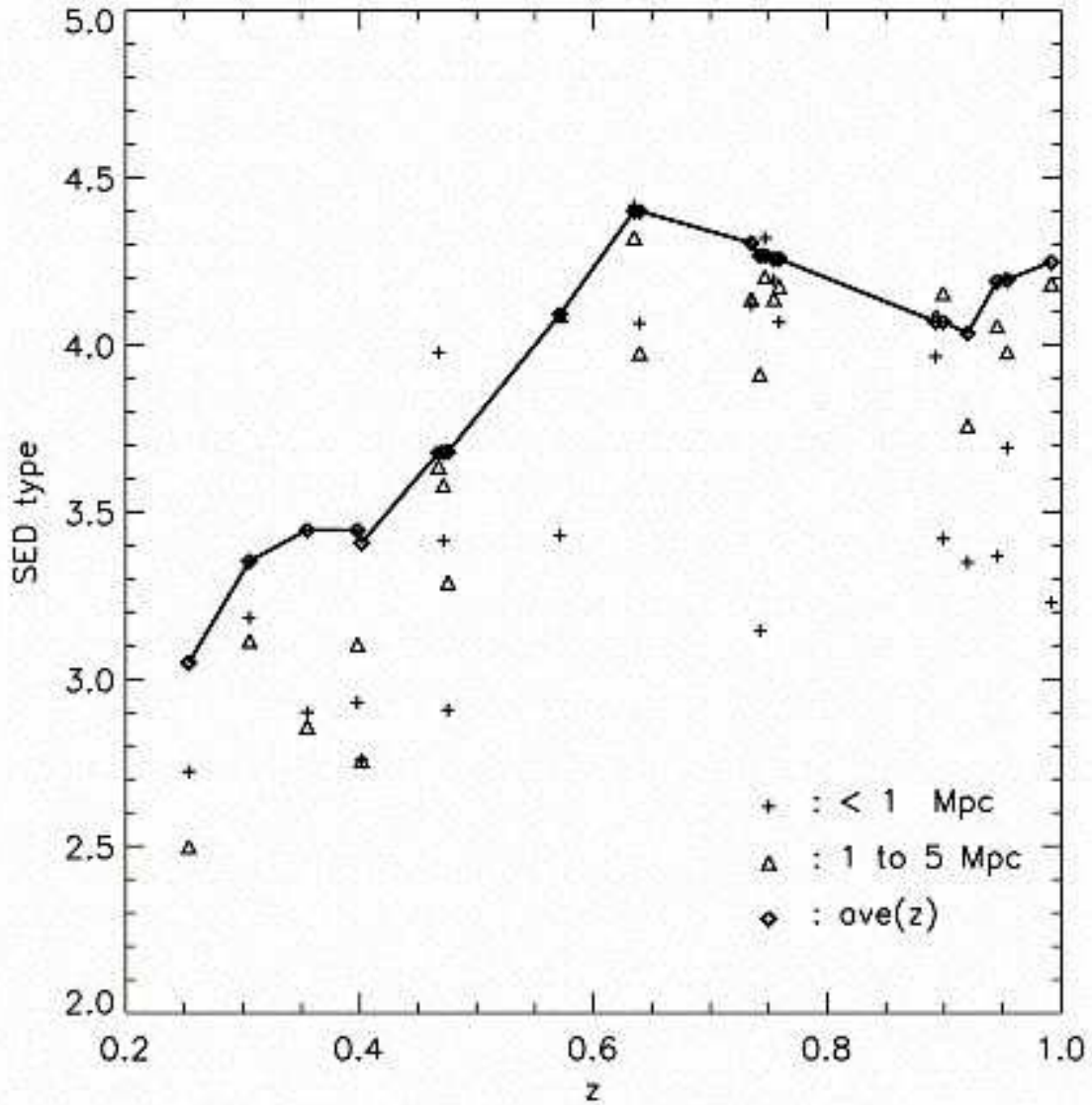
Fig. 12.— For each structure, the mean SED types of galaxies at projected R < 1\text{Mpc} and R = 1 to 5\text{ Mpc} are compared (solid line) with the mean type as a function of z (in a redshift bin \Delta z = 0.2 centered on the same redshift). One set of points is shown for each of the structures plotted at the mean redshift of each structure. Note the very pronounced trend for the central 1\text{Mpc} in the structures to have earlier mean SED type (low type) for the galaxies.
