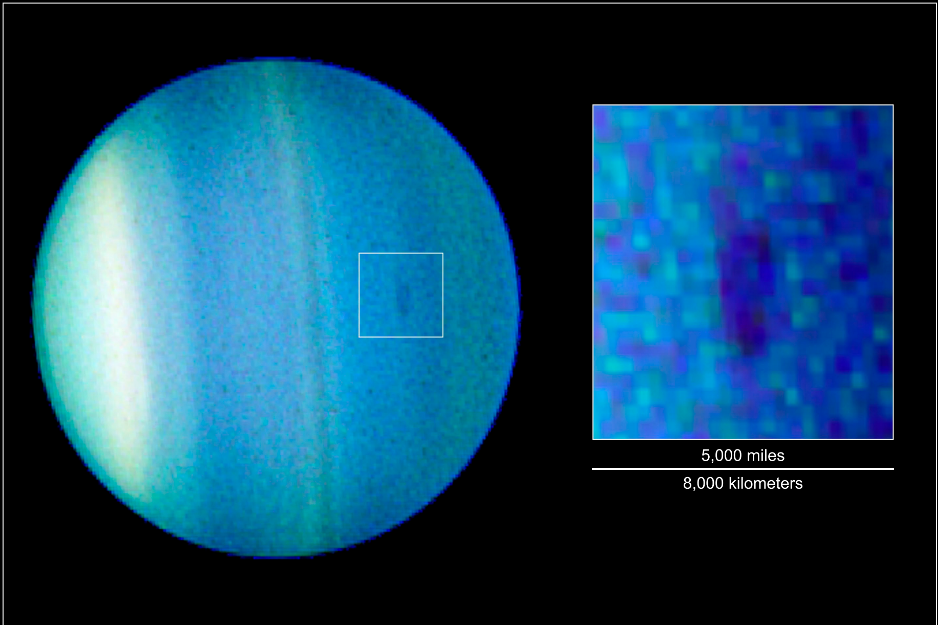
Uranus Dark Spot Hubble Space Telescope • Advanced Camera for Surveys
