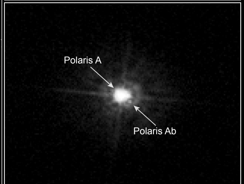
Polaris ■ \alpha Ursae Minoris Hubble Space Telescope ■ ACS/HRC
