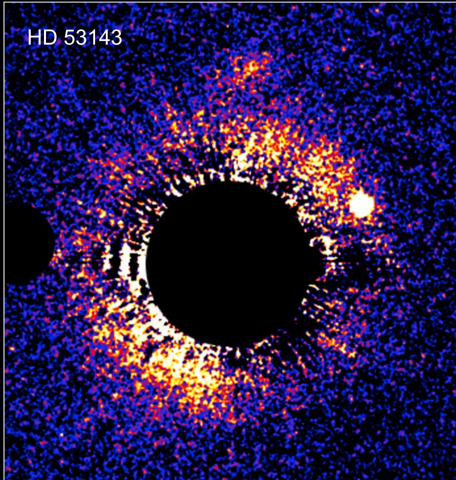
Circumstellar Debris Disks Hubble Space Telescope • ACS/HRC
