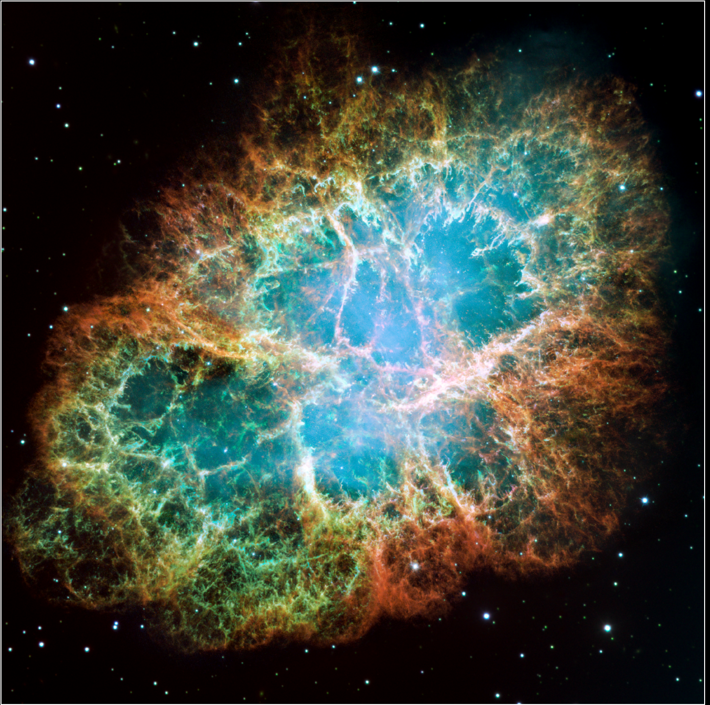
Crab Nebula • M1 Hubble Space Telescope • WFPC2
