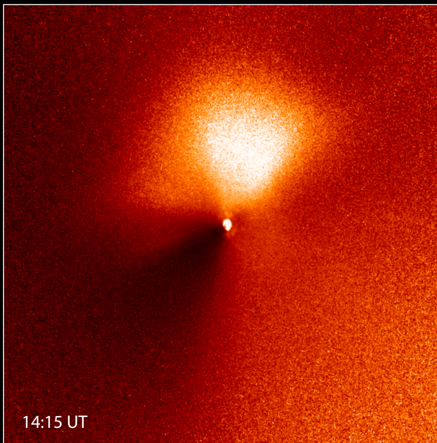
Comet 9P/Tempel 1 • June 14, 2005 Hubble Space Telescope • Advanced Camera for Surveys
