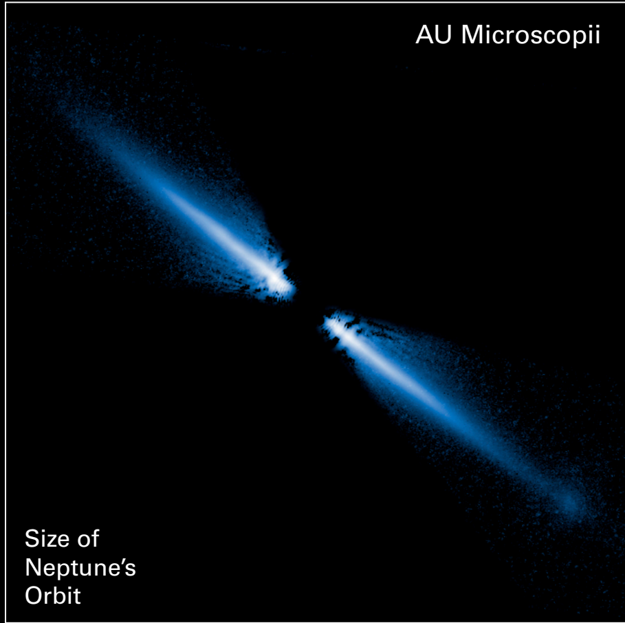
Size of Neptune's Orbit
