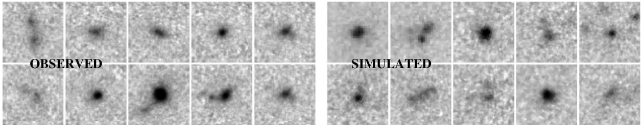
Fig. 1.— Postage stamps ( z_{850} images) of the 10 brightest ( 25.0 < z_{850,AB} < 27.2 ) i_{775} -dropouts from the UDF compared against a sample of HDF-N + HDF-S U -dropouts cloned (via no-evolution) to z \sim 6 and selected in a similar way. The high S/N of the UDF data is apparent. For context, the object in the upper right corner of the simulations is the familiar “quad” from the HDF-N (HDF4-858, Williams et al. 1996).
