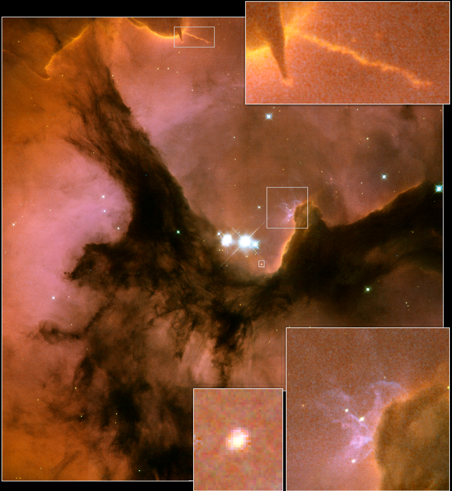
Trifid Nebula • M20 Hubble Space Telescope • WFPC2
