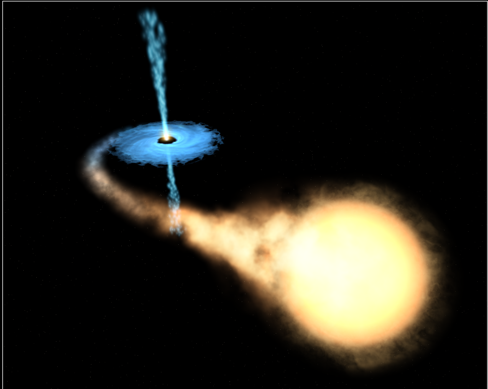
Artist's View of Black Hole and Companion Star GRO J1655-40
