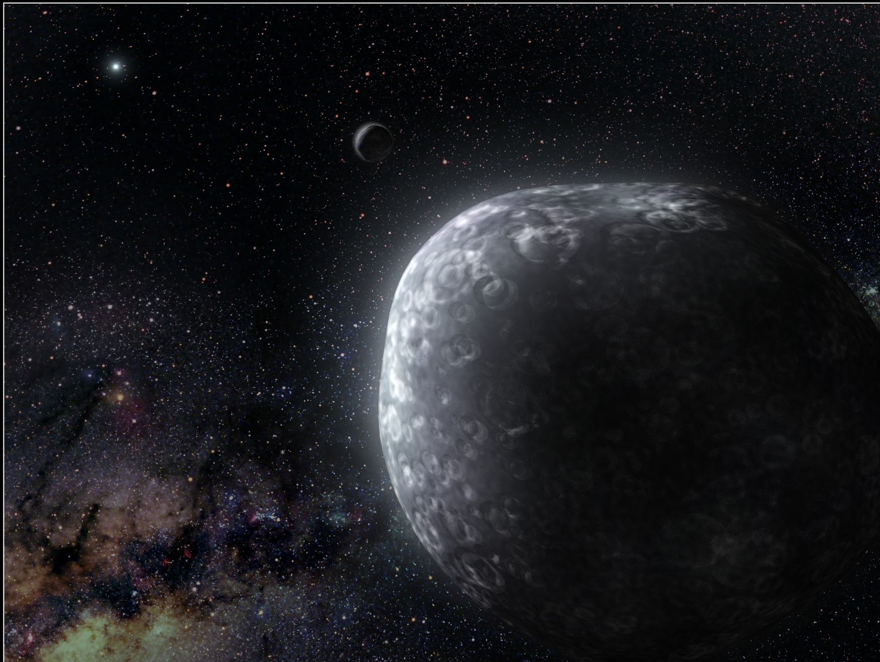
Artist's View of Kuiper Belt Object 1998 WW31
