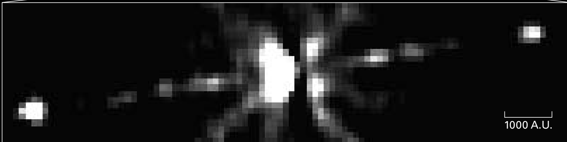
He2-90 Hubble Space Telescope • WFPC2
