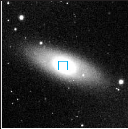
NGC 5838
