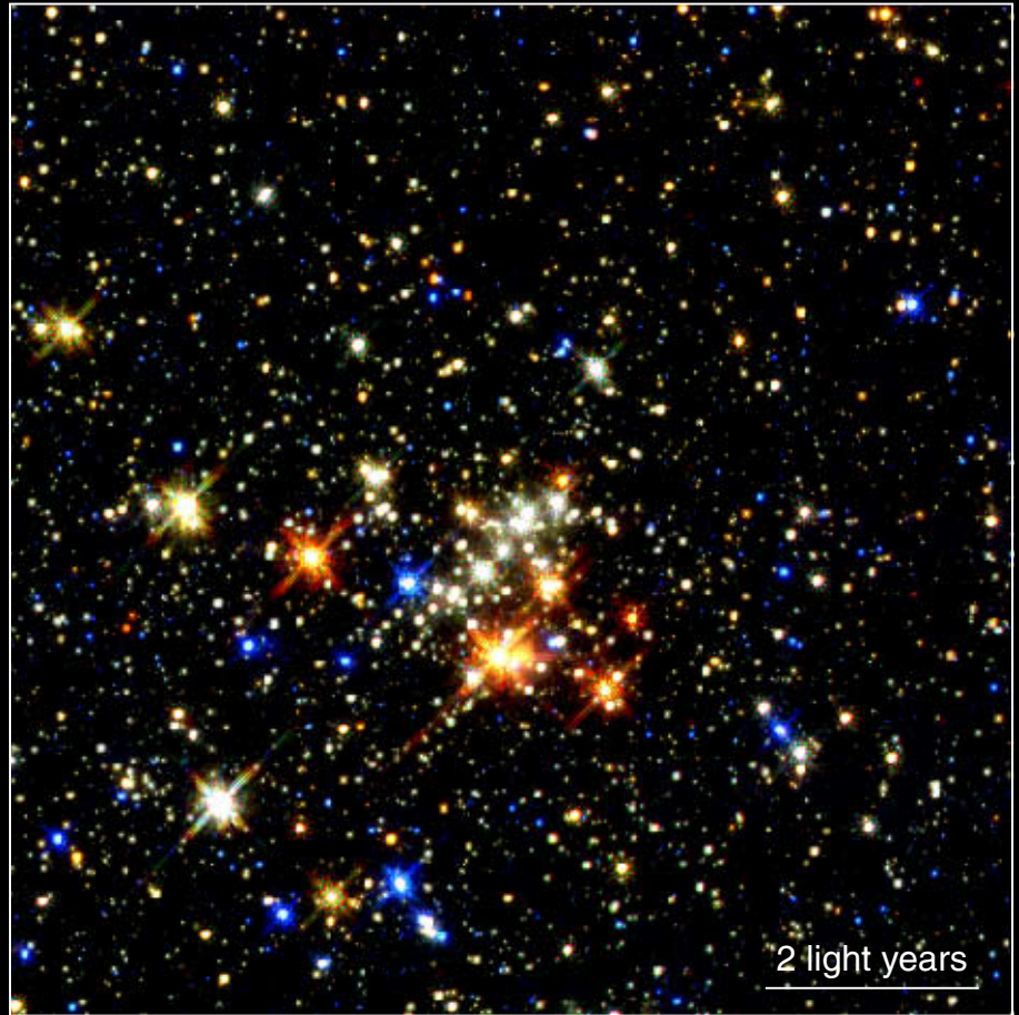
Quintuplet Cluster
