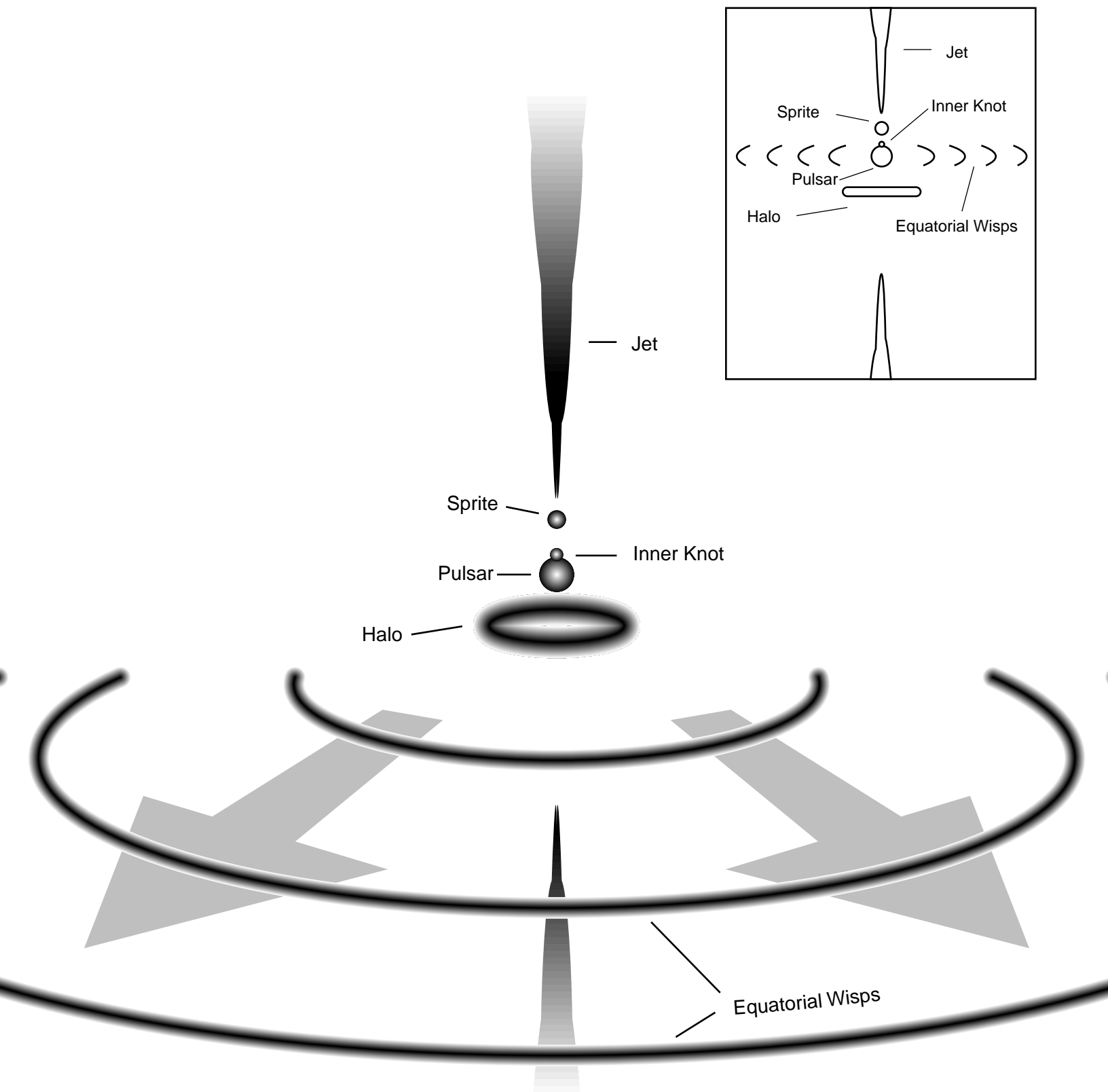
This is a diagram of environment around the pulsar at the heart of the Crab nebula, based on images take by Hubble Space Telescope. The jets of high speed particles, and the outward moving "equatorial wisps," are powered by the pulsar, which is the rapidly rotating crushed remnant of an exploded star.
