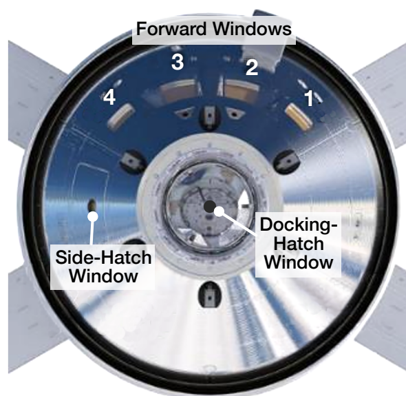
Figure 3.4: Orion Windows. Illustrative schematic of Orion showing the locations of Forward Windows 1–4, the docking-hatch window, and the side-hatch window.
