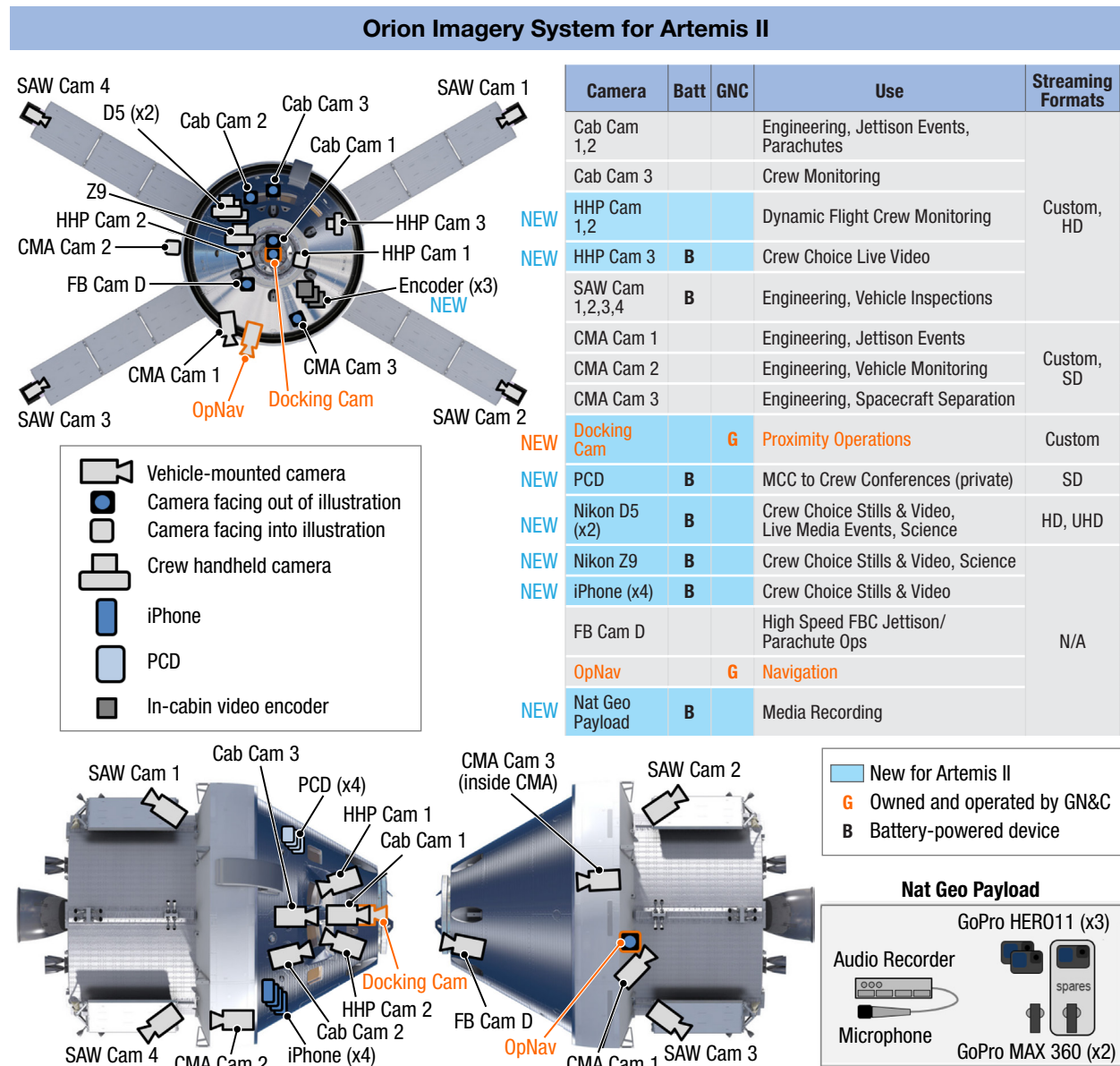
Figure 3.5: Orion Imagery System. The Orion imagery system configuration for Artemis II includes vehicle-mounted cameras used for monitoring spacecraft performance (exterior and interior to the crew cabin), crew handheld devices, navigation sensors, biomedical cameras, and the National Geographic public outreach payload. SAW Cam 3 and Cab Cam 2 had views of the Moon during the lunar flyby. Acronyms: HHP = Human Health and Performance; GN&C = Guidance Navigation and Control; CMA = Crew Module Adaptor; FB = Forward Bay.
