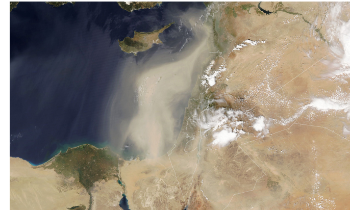
Dust storm from MODIS
