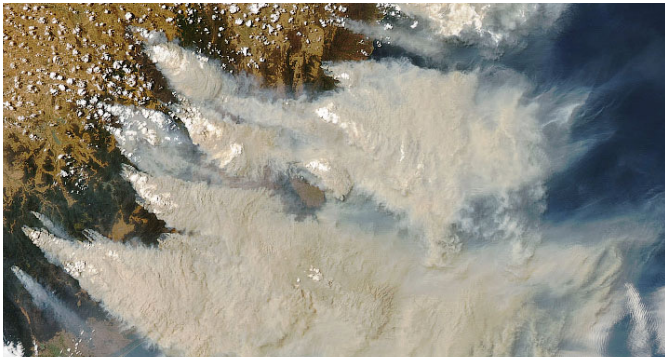
Fires and smoke from MODIS
