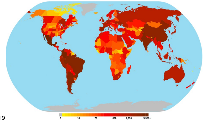
Users of CERES FLASHFlux data
