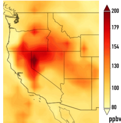
CO trends from AIRS and MOPITT
