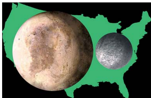
Pluto and Charon compared to the continental United States.
