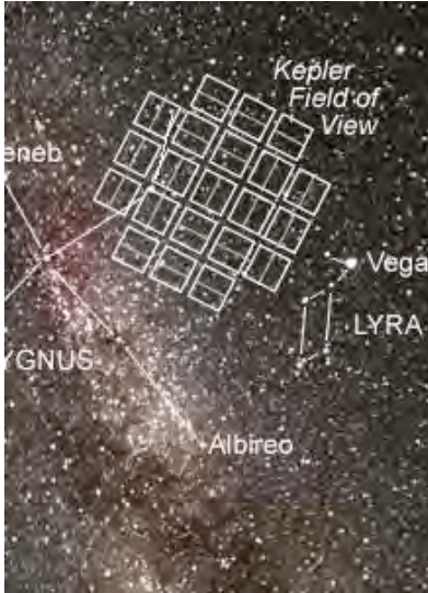
The Kepler Survey Field grid is located between the constellations Cygnus and Lyra. Although millions of stars are in this area, only 157,000 are studied by Kepler.
