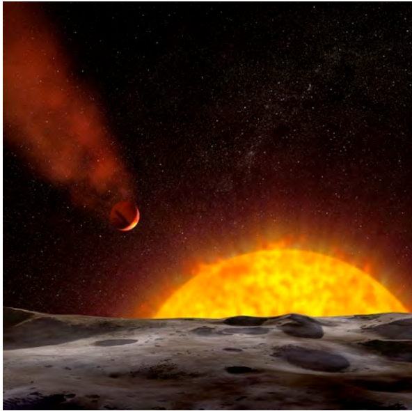
Artist view of planet G. Bacon (STScI/NASA)
