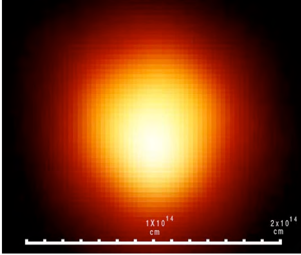
Betelgeuse (Hubble Space Telescope.) It is 950 times bigger than the sun!
