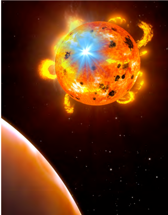
Artist rendering courtesy NASA/G. Bacon (STScI)
