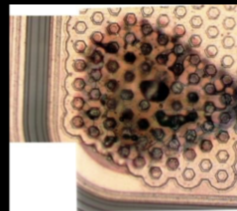
Destructive event in a COTS 120V DC-DC Converter
