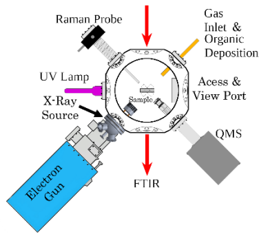
Above: ICEE UHV chamber showing radiation sources and in situ instruments.
