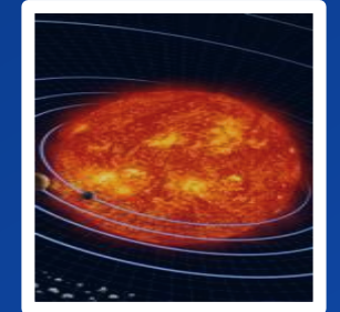
Heliophysics
