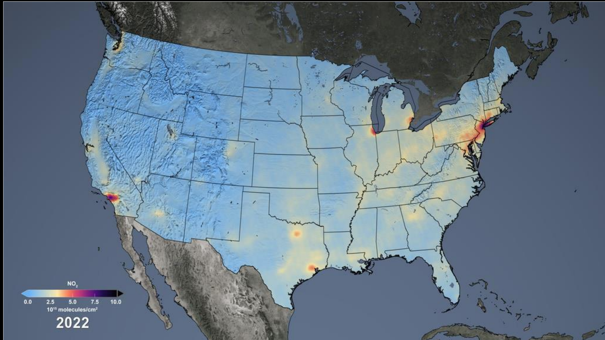
Average concentrations of NO 2 for 2022 over the U.S., as detected by the Ozone Monitoring Instrument on NASA's Aura satellite.
