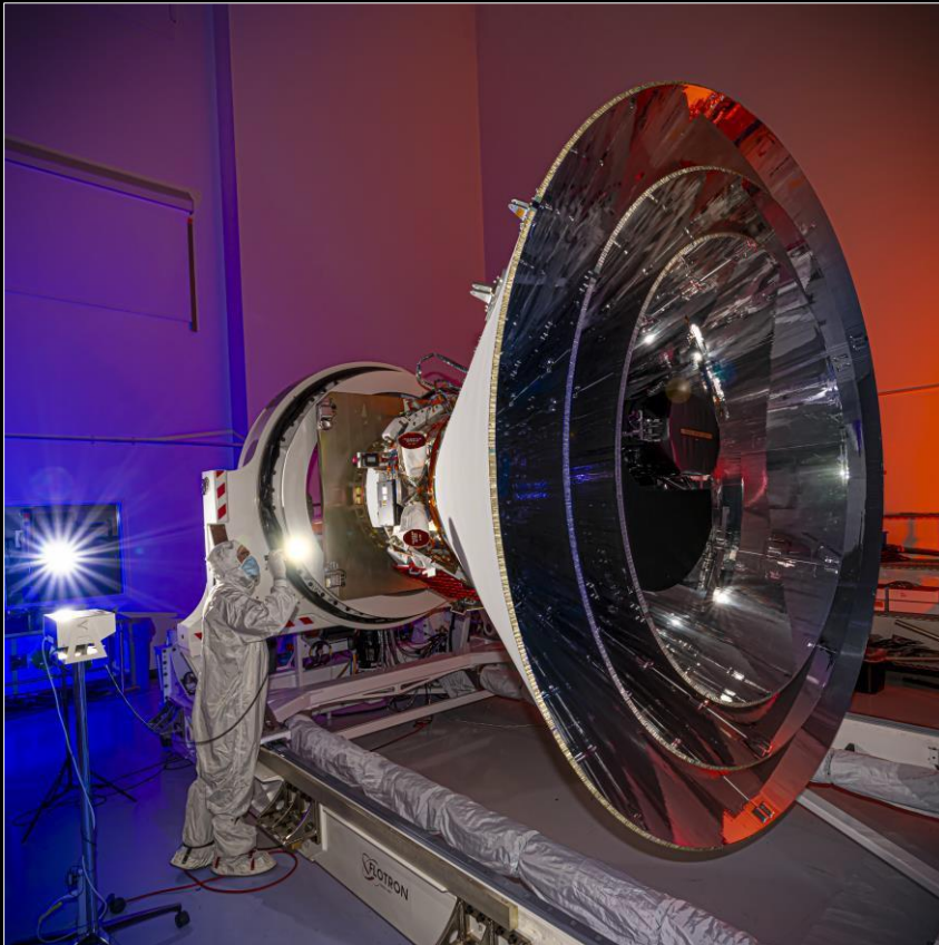
SPHEREx Observatory Assembled
