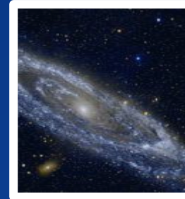
Astrophysics
