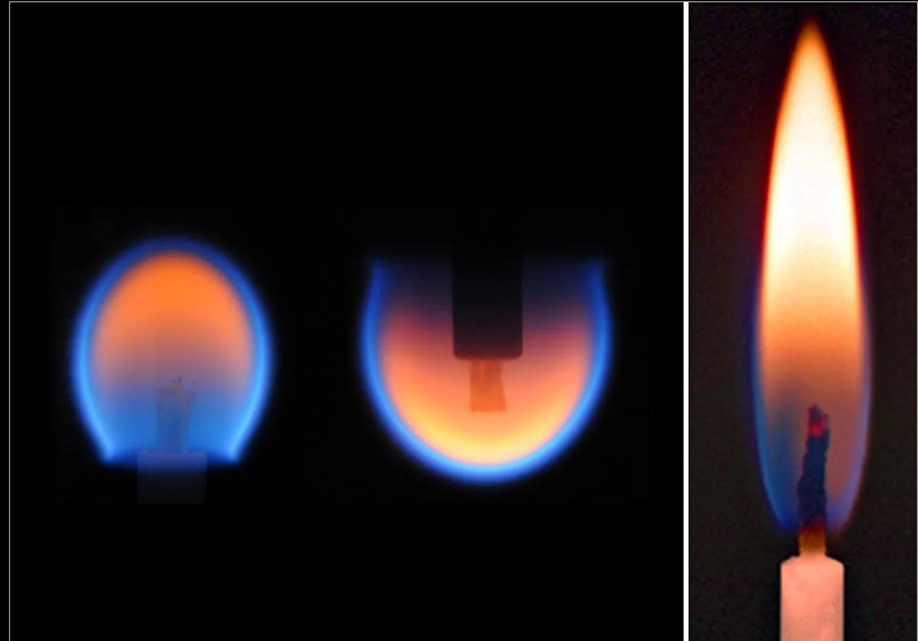
A spherical flame created in space (left), and a candle flame burning on Earth (right)
