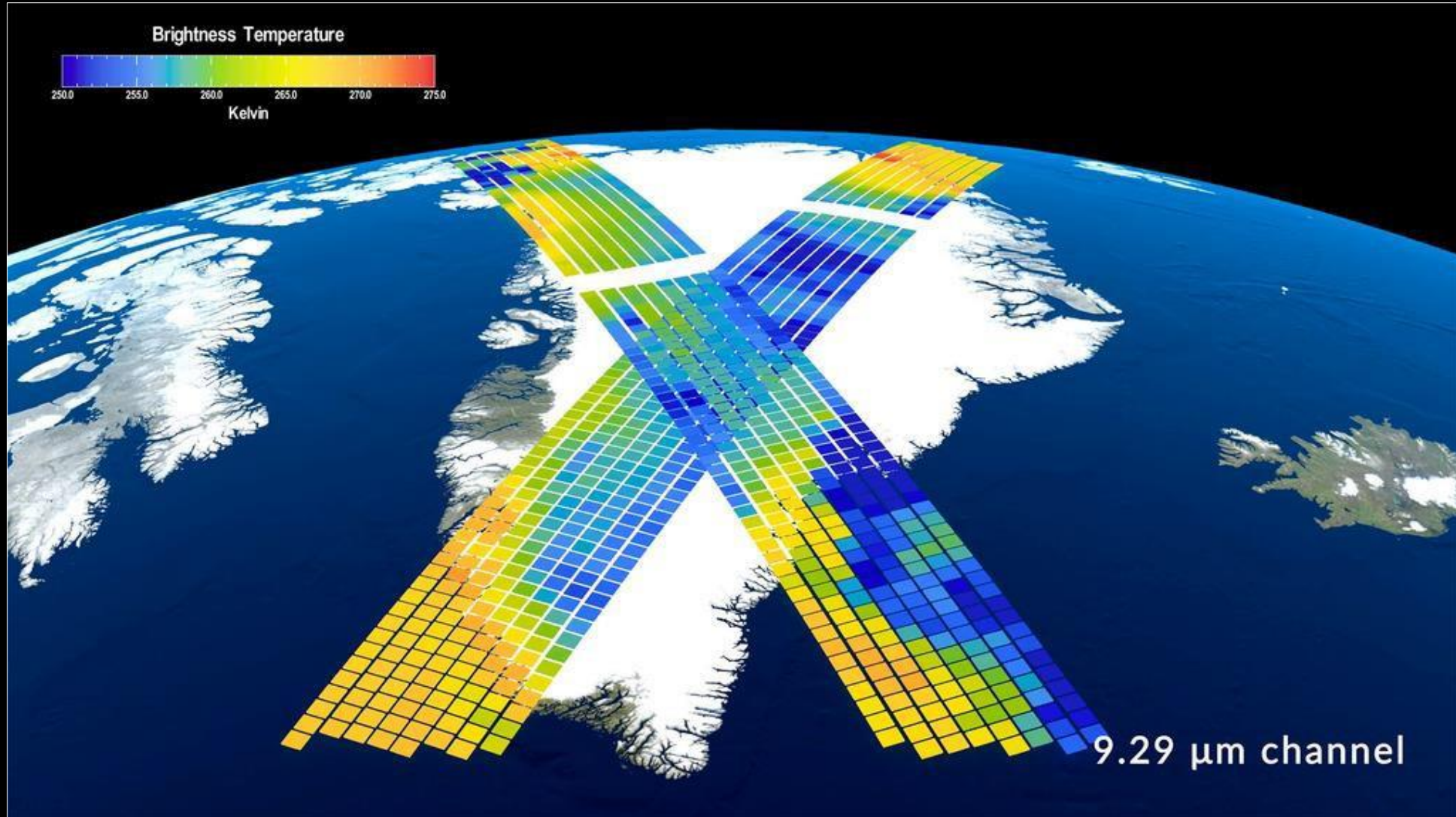
From a still frame of the PREFIRE first light video, showing a visualization of some PREFIRE-SAT2 data captured in July 2024.
