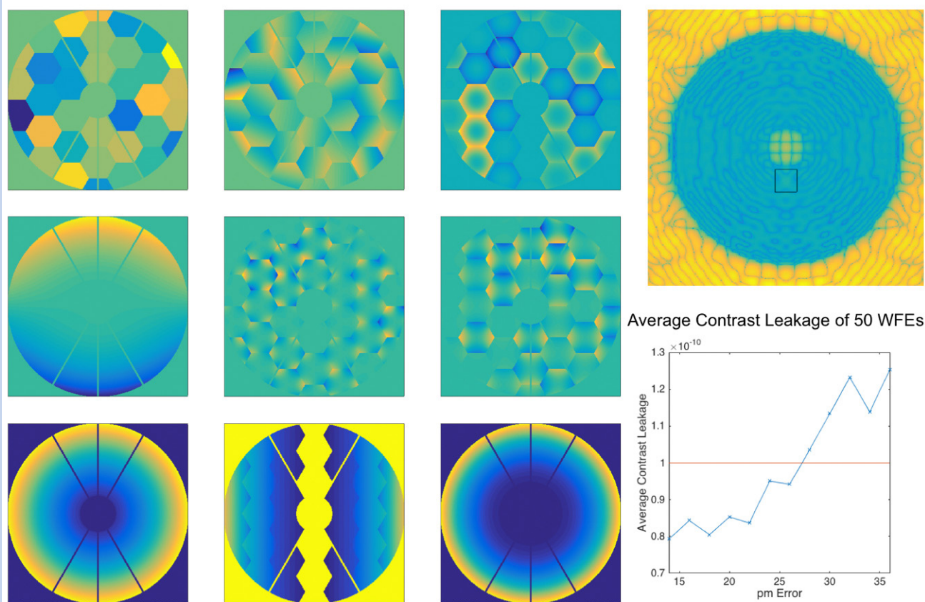
Fig. 7. Maximum amplitudes for each misalignment error are defined to be when the average contrast leakage over 4 to 6 \lambda/D regions of interest is 10^{-10} .
