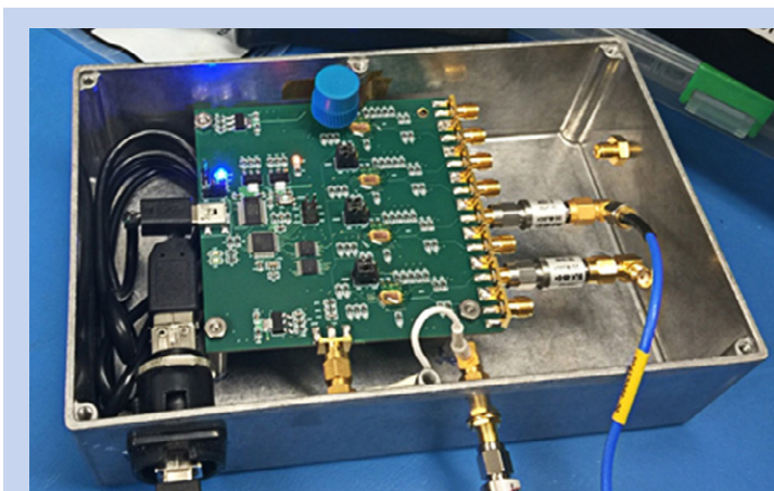
Fig. 11. The CMOS back-end is packaged in a robust housing that can be used for full receiver testing.
