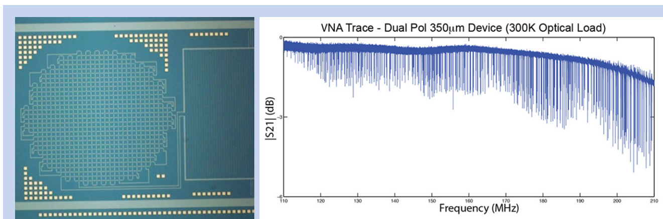
Fig. 1. Left: Micrograph of single detector (TiN KID) in an array tested on the CSO telescope in August 2014. The square grid with circular boundary at left is the photosensitive inductive element of the 540- \mu\text{m} -diameter KID, appropriate for a micro-lens-coupled device operating at 350 \mu\text{m} . Right: Vector Network Analyzer (VNA) “sweep” of frequency range occupied by the KIDs, showing absorbed power at the resonance of each of the \sim 500 detectors.
