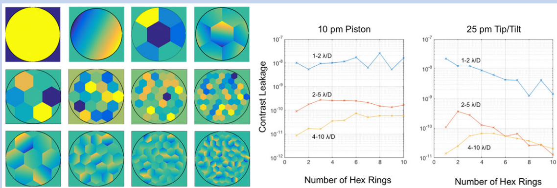
Fig. 6. 4 th -order coronagraph contrast leakage for piston and tip/tilt as function of segmentation.
