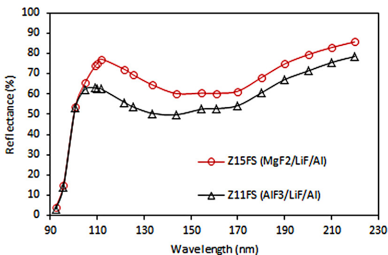
Fig. 5. FUV reflectance of tri-layer mirror samples from conventional evaporation.
