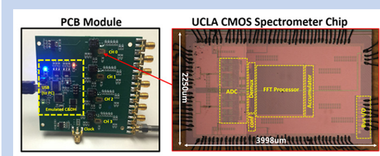
Fig. 10. Left: Photo of 4-pixel printed circuit board (PCB) module showing key circuitry. Right: Die photo of spectrometer processor CMOS SoC.
