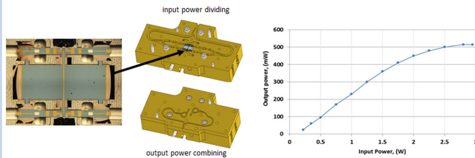
Fig. 5. Performance of the 4-way-power-combined first-stage tripler. Due to the increased input power levels available at 70-75 GHz, this single chip can produce over 500 mW at 211 GHz, a new world record.
