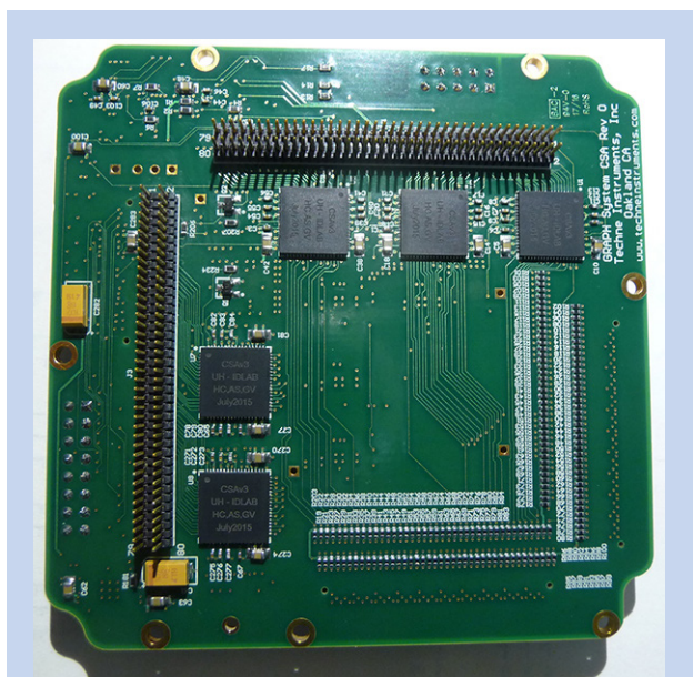
Fig. 11. 50-mm detector amplifier board with 10 CSAv3 chips, five on a side.
