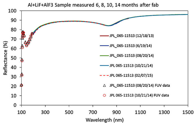
Fig. 3. Measured reflectance of a bi-layer-protected Al mirror sample ( \text{AlF}_3 +LiF on Al) measured 6, 8, 10, and 14 months after fabrication showing excellent stability. Results over the FUV to NIR spectral range.
