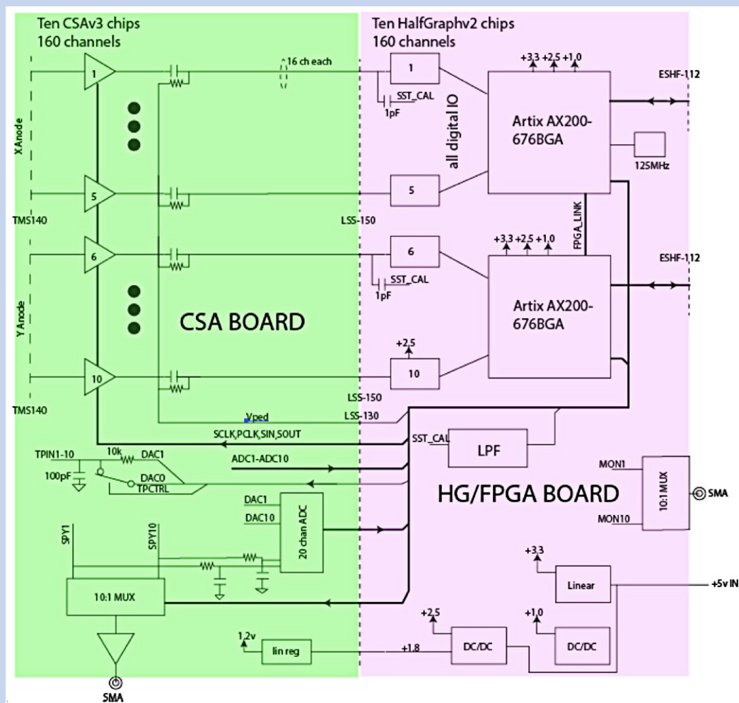
Fig. 9. High-level schematic of 50-mm detector electronics. 160-channel amplifier board (left) and 160-channel digitizer board with two FPGAs to control ASICs and calculate event centroids (right).
