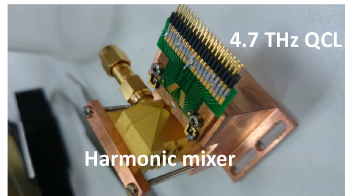
Array of DFB lasers at ~4.7 THz. The harmonic mixer is used to phase-lock the QCL LO.
