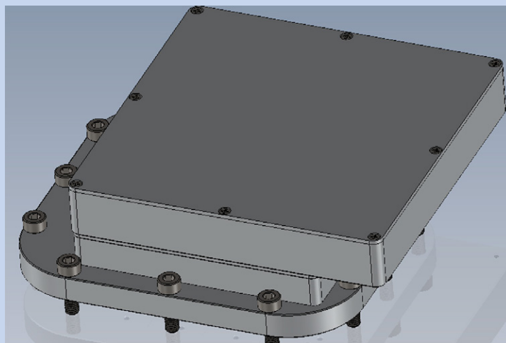
Fig. 10. Rendering of two electronics boxes (amplifier and digitizer) mounted to 50-mm detector backplate.
