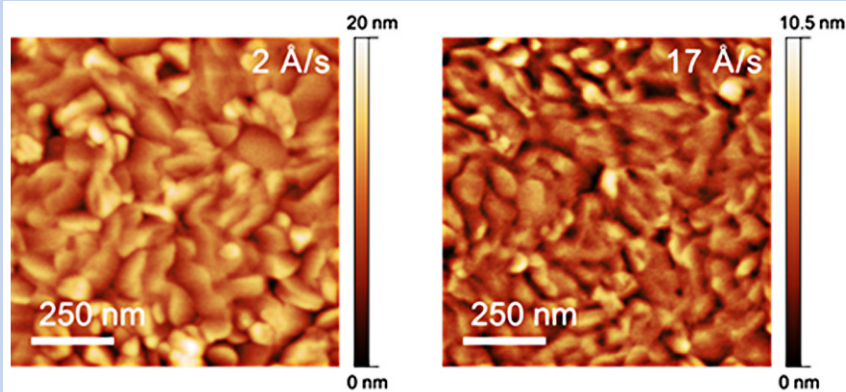
Fig. 12. AFM images of UHV electron beam evaporated Al films (60-nm thickness) at deposition rates of 2 Å/s (left) and 17 Å/s (right) at a length scale of 1 \mu\text{m} .
