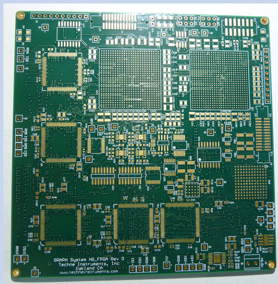
Fig. 12. 50-mm detector digitizer board with 10 HalfGRAPH2 chips, five on a side.
