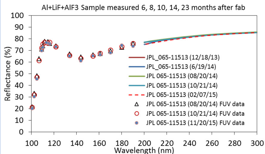
Fig. 4. Measured reflectance of a bi-layer-protected Al mirror sample (AlF 3 +LiF on Al) measured 6, 8, 10, 14, and 23 months after fabrication showing excellent stability. Expanded view showing the FUV spectral range.
