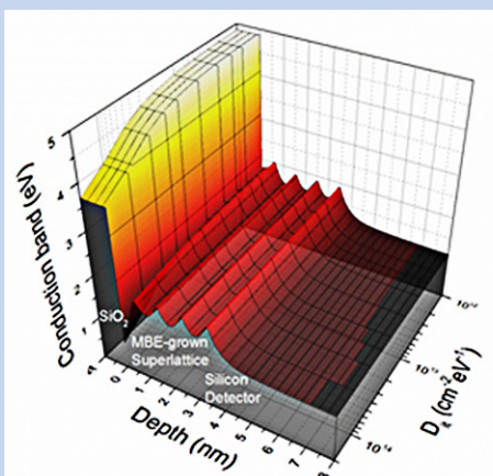
Fig. 1. Left: Band diagram of a SL-doped silicon surface. Right: JPL's 8"-wafer-capacity silicon molecular beam epitaxy (MBE) facility, where SL doping is performed.
