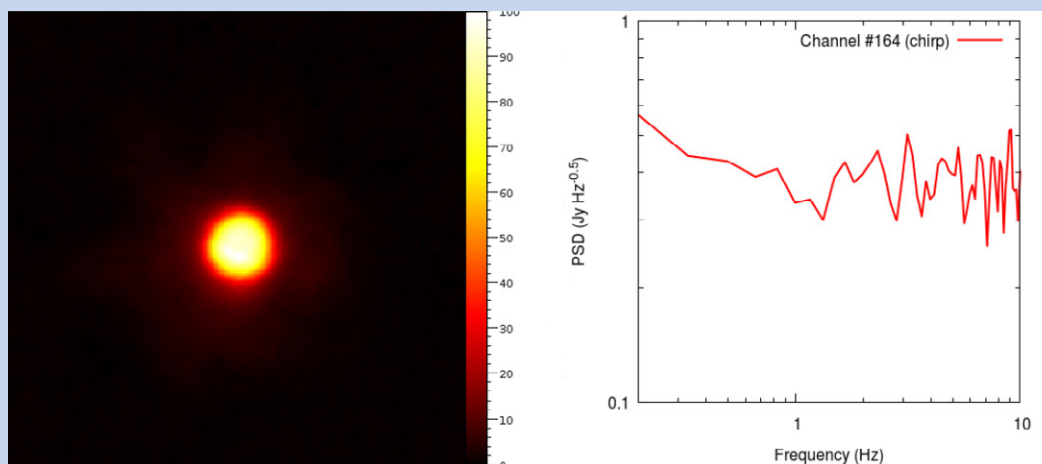
Fig. 6. Left: Image of Jupiter at 350\ \mu\text{m} acquired with CSO demonstration camera and chirped readout. Right: Noise spectrum of KID read with chirp technique, demonstrating low 1/f noise (PSD, power spectral density).
