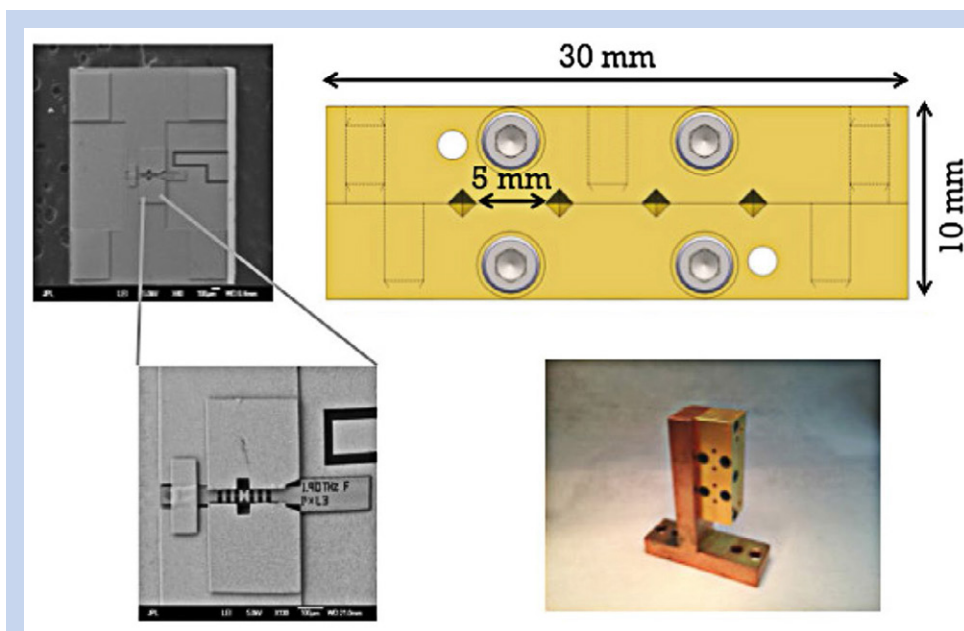
Fig. 9. Left: Mixer chip and silicon micro-machined substrate used to mount it. Top right: Schematic of the completed 4-pixel mixer module. Bottom right: Picture of the mixer module.
