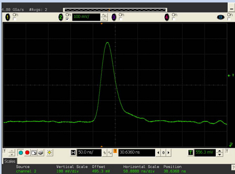
Fig. 4. Amplifier response to 50-fC input pulse with a 5-pF load. Note the 20-ns rise time and a return to baseline in 75 ns while retaining a noise value of \sim 1000\text{ e}^- \text{ rms} .
