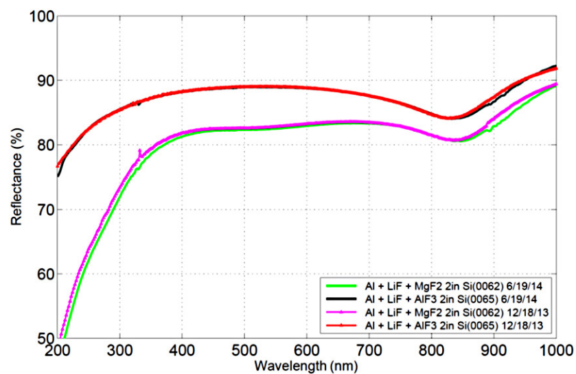
Fig. 2. Reflectivity of Al+LiF mirror samples with \text{MgF}_2 and \text{AlF}_3 protective layers. Measured six months after fabrication, these samples show little degradation.
