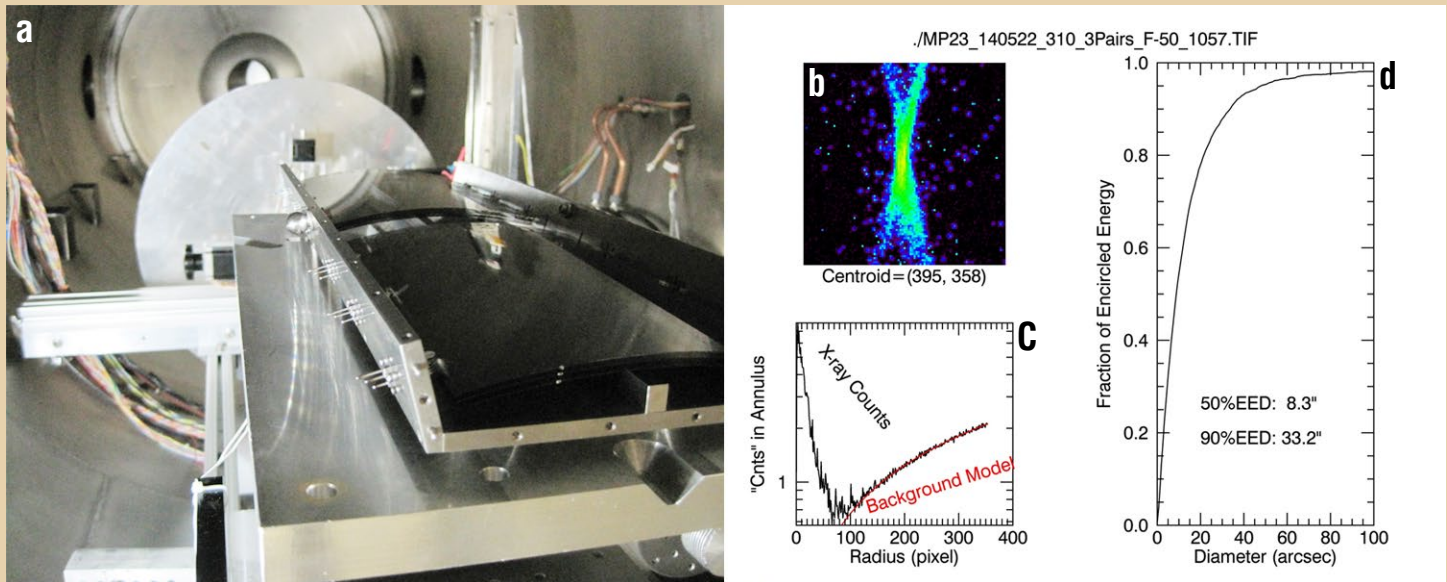
Fig. 1. (a) A representative TDM containing three co-aligned and bonded primary-secondary (paraboloid-hyperboloid) mirror pairs, shown in an X-ray chamber for full-illumination testing; (b) TDM X-ray image at 4.5 keV, displayed in a logarithmic scale to clearly show image shape; (c) Details of background analysis of image (b); (d) Encircled energy vs. diameter, showing HPD of 8.3 arcsec and 90%-encircled-energy diameter of 33.2 arcsec.
