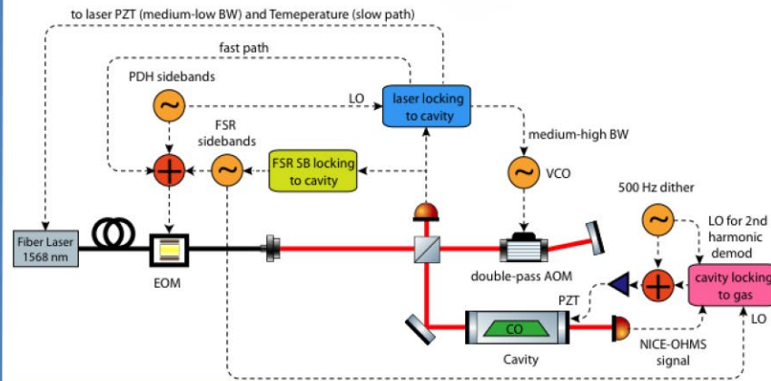
Stanford laser stabilization system showing feedback loops
