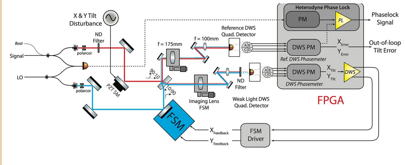
Fig. 2. The dedicated DWS test-bed has a primary and reference signal path as well as a fast steering mirror (FSM) for closed loop control (FPGA, field programmable gate array; ND, neutral density; PM, Phase Meter; SM, Steering Mirror).
