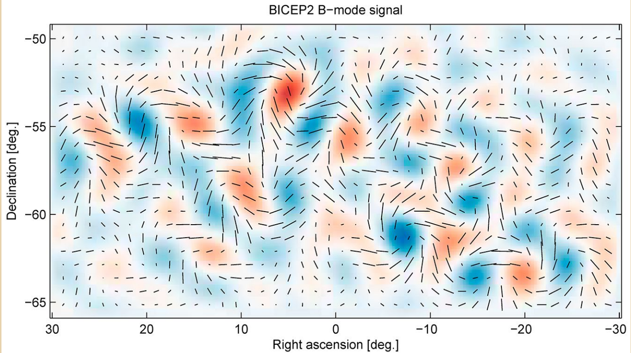
Fig. 2. B-mode polarization pattern measured by the BICEP2 instrument at 150 GHz. The blue and red coloration indicates the (positive and negative) B-mode amplitude, corresponding to clockwise and counter-clockwise spiral polarization patterns, respectively. The measurement was obtained in three years of observations, using a focal plane array of planar antenna-coupled bolometers similar in design to devices being developed through this SAT program.
