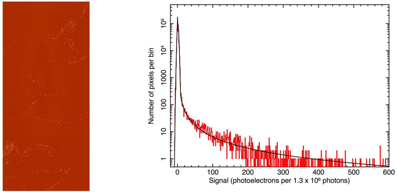
Fig. 4. Left: Image obtained from by CCD with a 220 nm-thick OBF illuminated with 1.3 \times 10^6 photons/pixel of 800 nm light. Pinholes (white spots) are evident. Right: Histogram of amplitudes of the 440,000 pixels in the image on the left. While 99% of pixels are in the peak, and are consistent with zero amplitude, about 1% of pixels show transmission greater than 10^{-6} .
