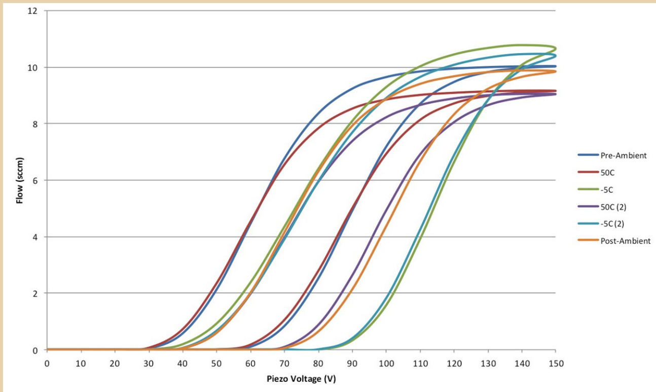
Fig. 6. Graph of prototype microvalve flow rate vs. driving voltage before and after various thermal conditions. The pre- and post-test curves at ambient temperature show an approximate 10 V shift in the response curve, still within alignment requirements. The next set of microvalves will include an additional staking step to help reduce this shift.
