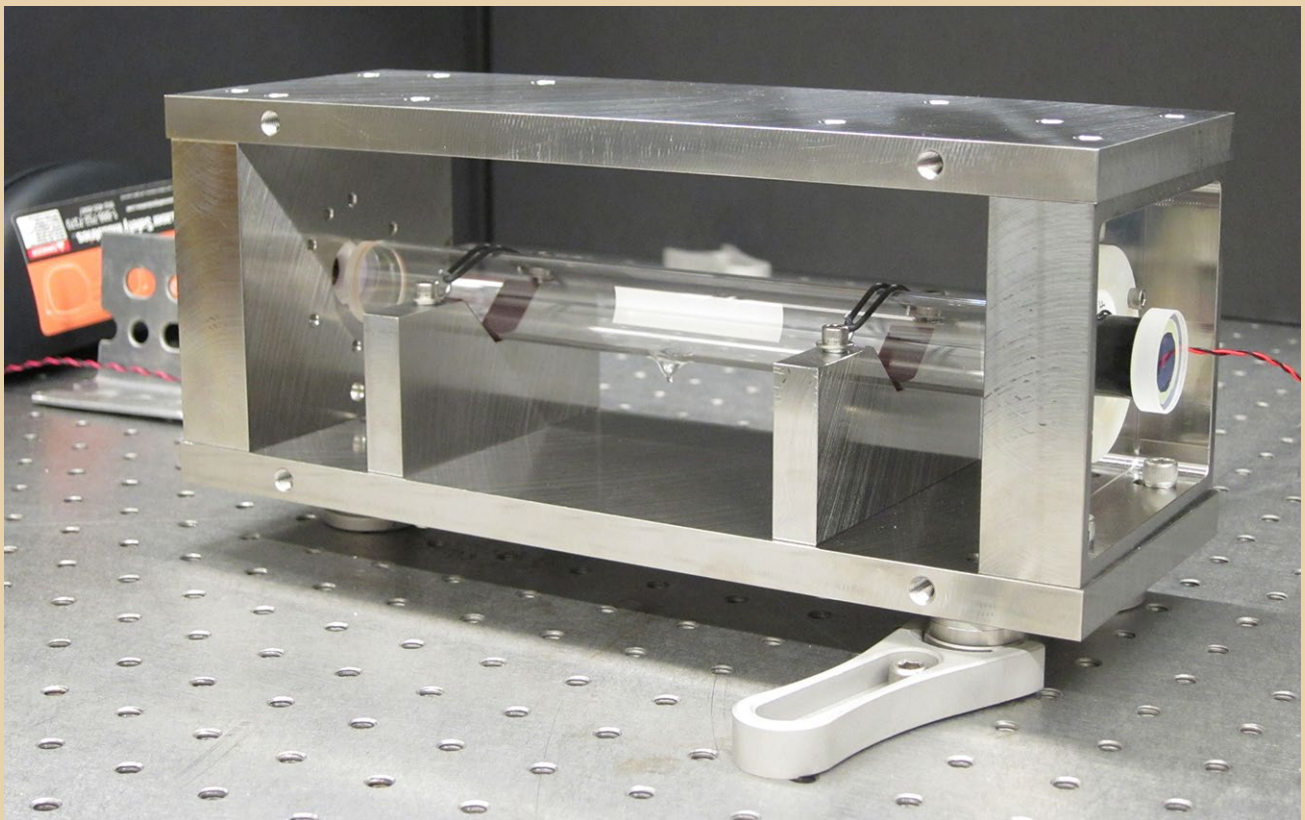
Fig. 1. Optical cavity #1.
