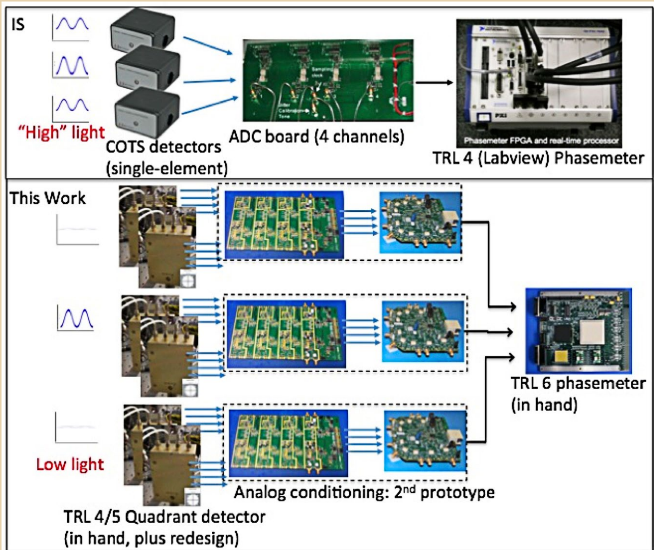
Fig. 1. End-to-end testing of component prototypes in a modified test-bed represents a significant step in system-level maturity of the Phase Measurement System, raising it from TRL 4 to TRL 5 (COTS, commercial off the shelf; ADC, analog to digital converter).
