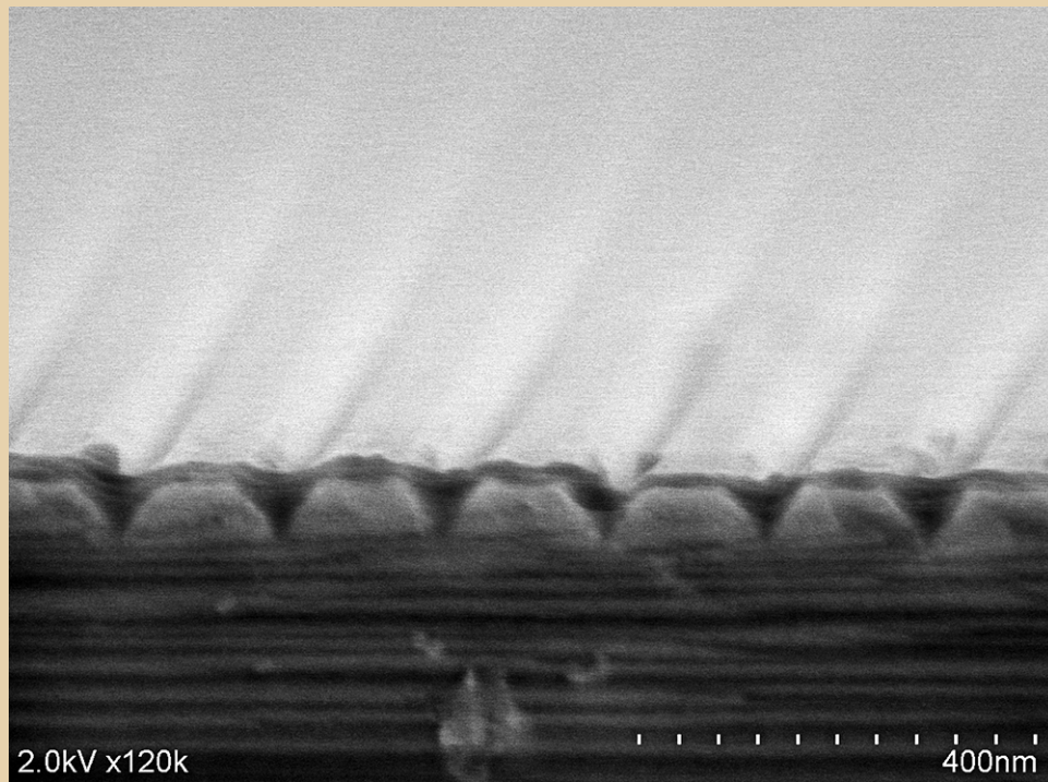
Fig. 2. SEM image of a cleaved \langle 100 \rangle wafer following our etch recipe. The trapezoidal groove features with smooth sidewalls are created by KOH etching to the \langle 111 \rangle planes.
