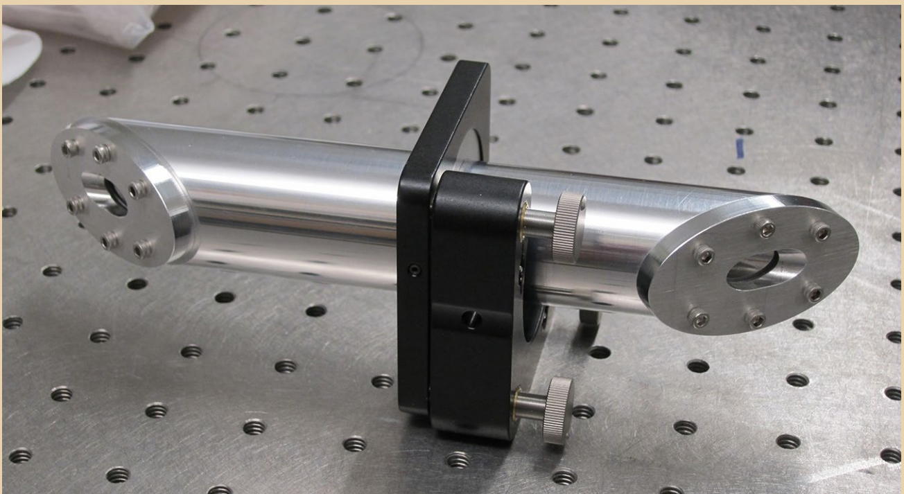
Fig. 2. Brewster cell.
