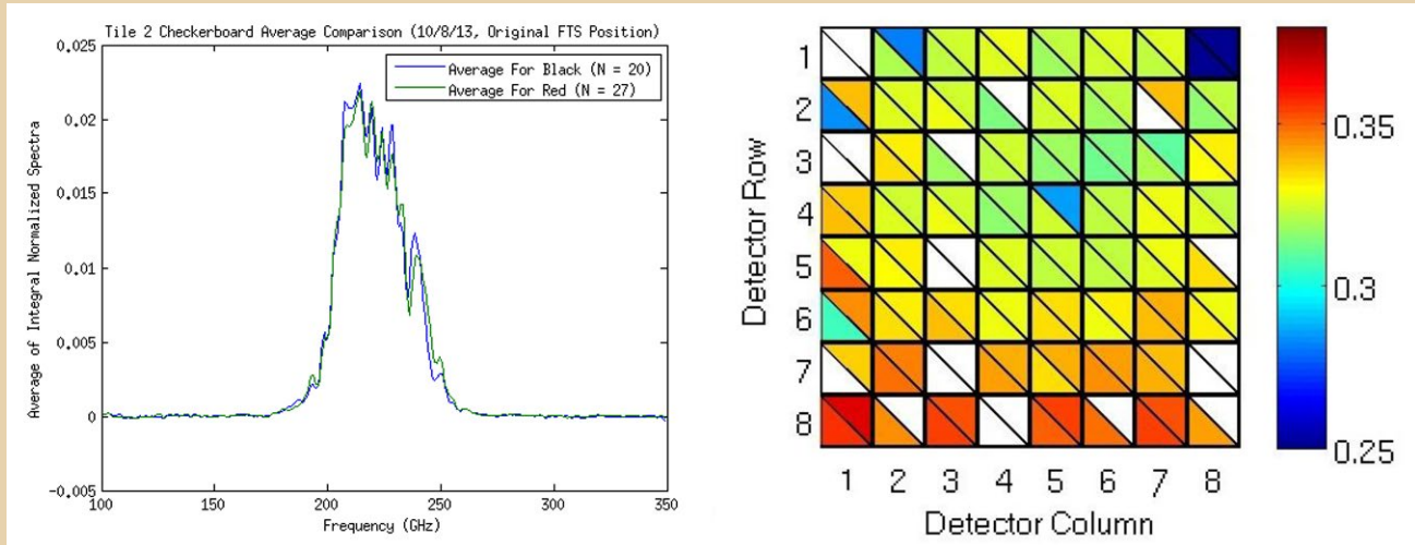
Fig. 4. Left: Spectral response for a new 220 GHz antenna-coupled TES bolometer array, giving the desired bandwidth and center frequency. Right: The system optical efficiency of the antenna-coupled devices plus window and blocking filters is 30-35%, comparable to the efficiency achieved in arrays operating at 95 and 150 GHz.
