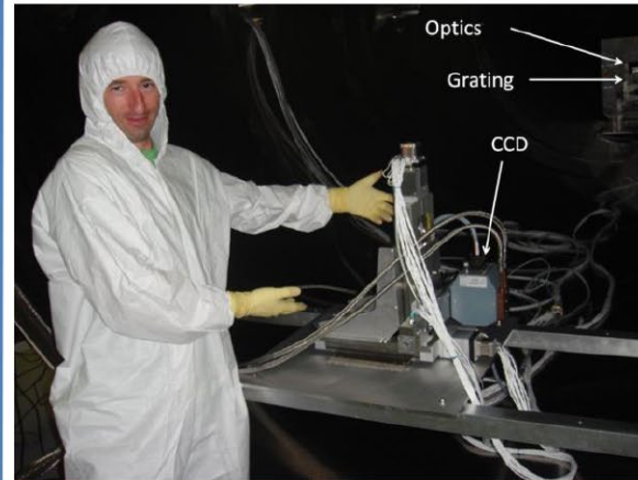
Resolution testing at NASA/MSFC
