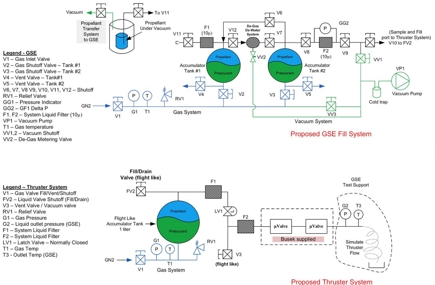
Fig. 4. Schematic of GSE (top) and colloid thruster feed system (bottom) showing all necessary components for drying, filling, and draining propellant from the new tank and feed system. All parts have been procured and will undergo testing in Fall 2014.
