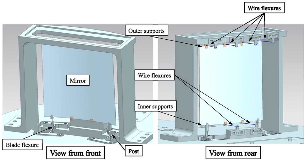
Fig. 3. Mirror segment mounting scheme.
