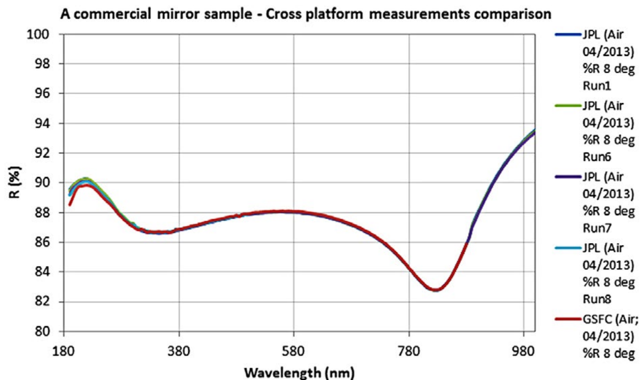
Figure 3. A cross platform measurement of reflectance of a commercial mirror sample showing excellent agreement between measurements made with two different instruments.
