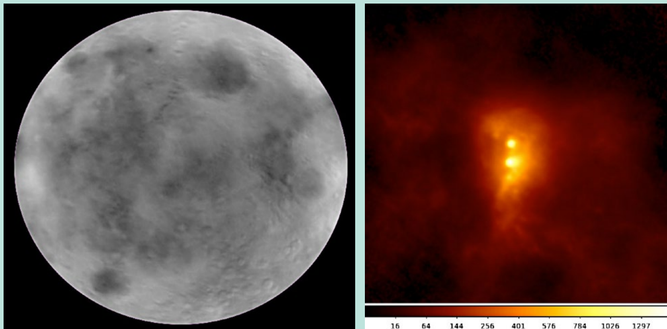
Figure 4. LEFT: Image of the moon, obtained using MAKO at the CSO. RIGHT: MAKO image of Sagittarius (Sgr) B2, a region of massive star formation located ~200 parsecs (pc) from the galactic center. The three well-known bright cores—Sgr B2(N), Sgr B2(M), and Sgr B2(S)—are visible at the center of the image and correspond to dense concentrations of interstellar dust heated by the newly formed stars. Fainter extended emission from the larger molecular cloud region is also visible. The MAKO Sgr B2 image corresponds quite well with an image of the same region obtained using SHARC-2.
