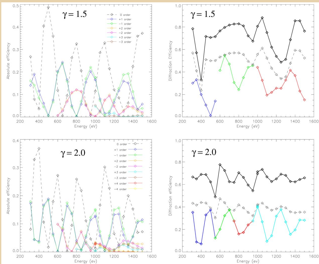
Figure 2.5-1. Upper left and right: These plots show results at a graze angle of 1.5°. Lower left and right: These plots pertain to a graze of 2°. Left column: These plots give the absolute efficiencies (inclusive of the reflectivity of Au at the appropriate graze) as a function of energy for all measurable orders. Right column: These plots give the efficiencies summed over available orders: blue = 1 st order; green = 1 st + 2 nd ; red = 1 st + 2 nd + 3 rd ; cyan = 1 st + 2 nd + 3 rd (+ 4 th ); dashed black = 0 th + 1 st + 2 nd + 3 rd (+ 4 th ). The solid black lines show the relative efficiency (absolute efficiency divided by Au reflectivity at the appropriate \gamma ).
