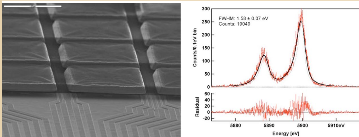
Figure 2.6-1. Left: This scanning electron microscope image of a PSA prototype array shows the close-packed pixels that are on a 75 micron pitch. Right: Shown here is a spectrum from one of the pixels of the type shown at left when a pixel is illuminated with X-rays from a ^{55}\text{Mn} source.
