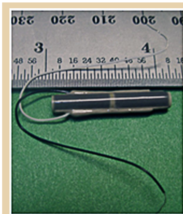
Figure 2.7-1. Electrostrictive adjuster manufactured by Xinetics. When voltage is applied to the device, the length changes. The change in length is stable when the voltage is removed.
