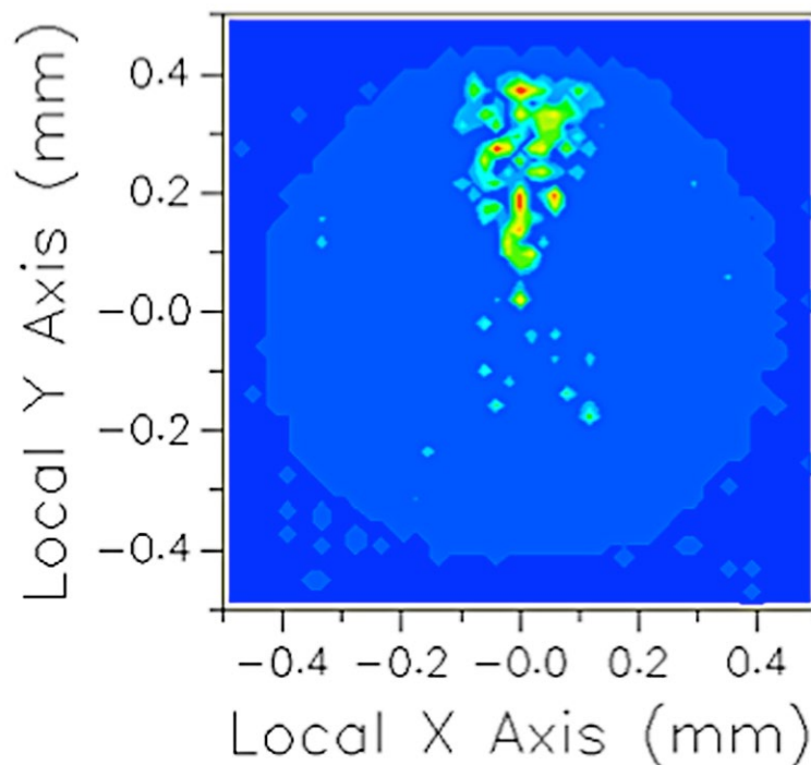
Figure 2.2–4. Power scattered onto the main science detector from a hole in the secondary mirror. Total power is 6 \times 10^{-11} W, and 0.93 W is delivered to the sky.
