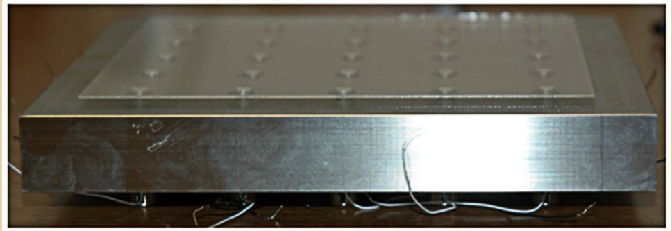
Figure 2.7-5. Flat mirror test fixture. Glass flat attached to 25 of the adjusters at the top, with the titanium reaction structure on the bottom.
