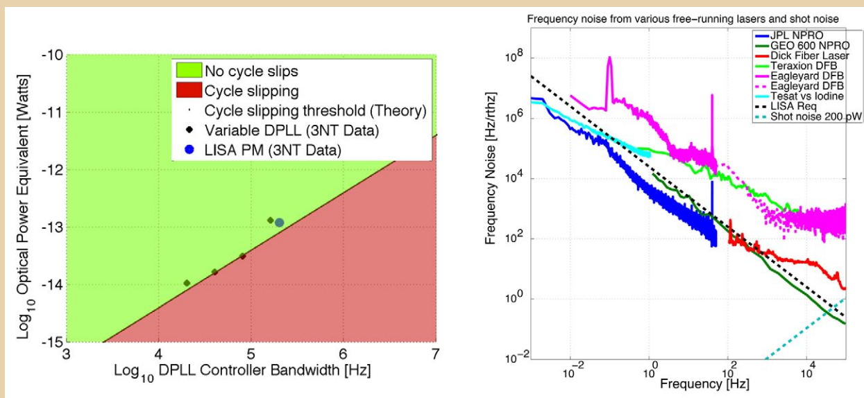
Figure 2.1-3. An analytic model of the phasemeter was developed that shows: Left: the interplay between received signal power and phase lock loop bandwidth. Laser frequency noise sets the limit on how low this bandwidth can be. Right: Noise from several lasers is shown, with several measurements limited by measurement noise.
