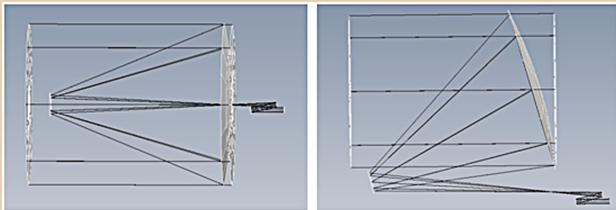
Figure 2.2-1. Left: NGO on-axis Cassegrain design. Right: NGO off-axis Cassegrain design.
