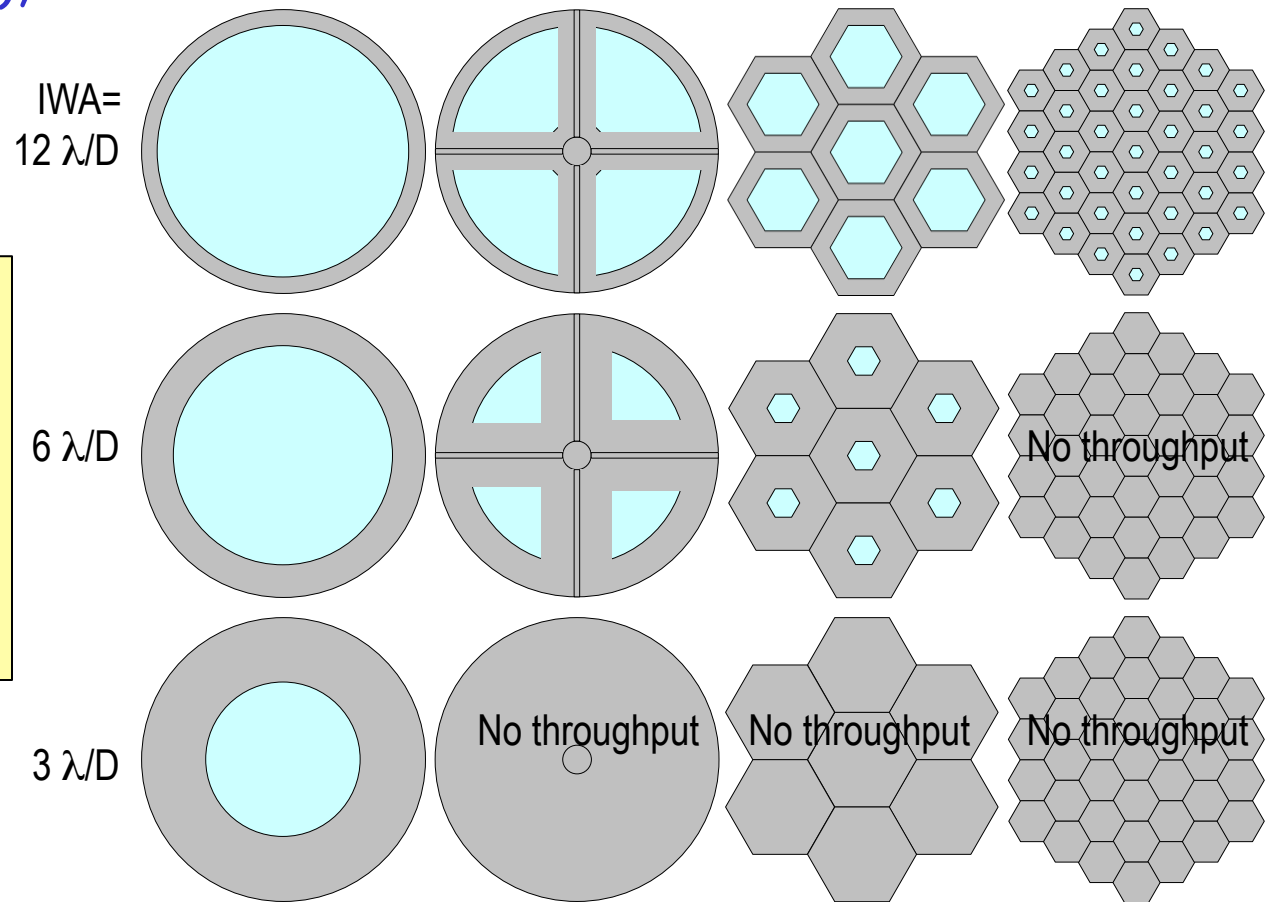
Masking in Lyot stop for various obscurations and segmentations
